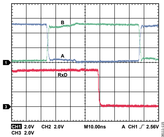
Figure 15. ADM2582E Receiver Propagation Delay
