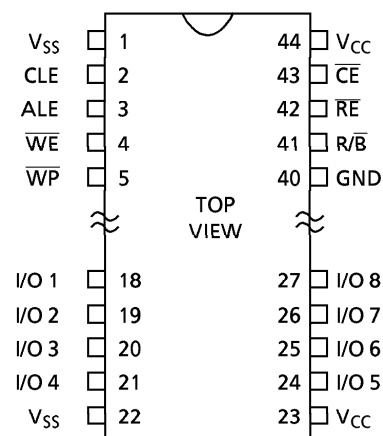
Figure 1. TC5816 Pinout
