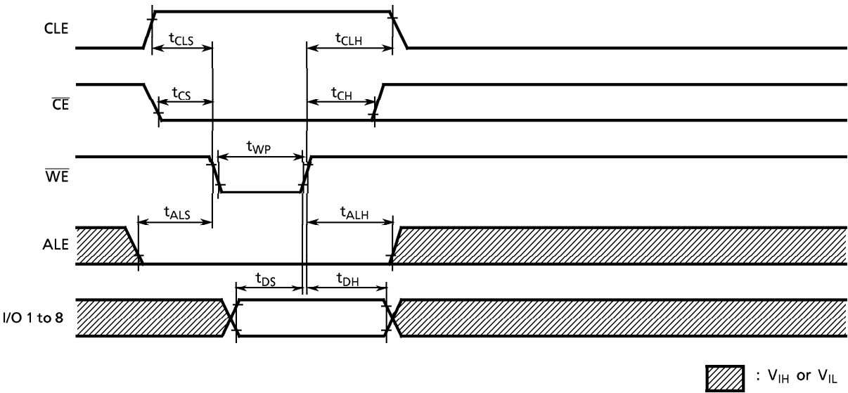
Command Input Cycle Timing Diagram
