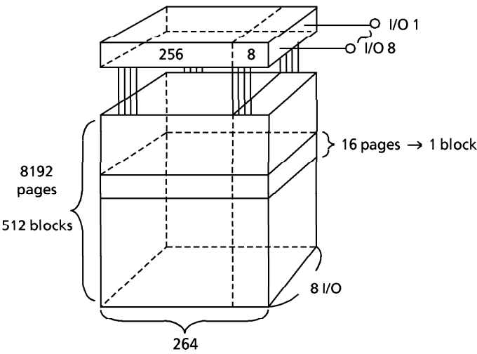
Figure 2. TC5816 Schematic Cell Layout
