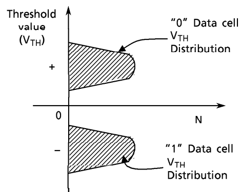
Figure 19. V_{TH} Distribution for “0” and “1” data cells
