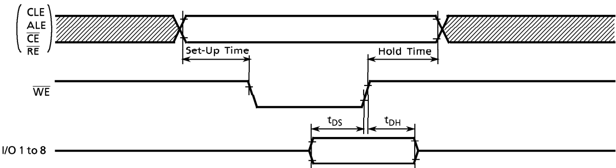
Latch Timing Diagram for Command/Address/Data
