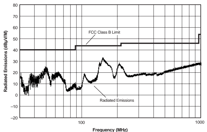
BWR-15/165-D48 Radiated Emissions FCC Part 15 Class B, 3 Meters Converter Output = \pm 15\text{Vdc} @ \pm 132\text{mA}
