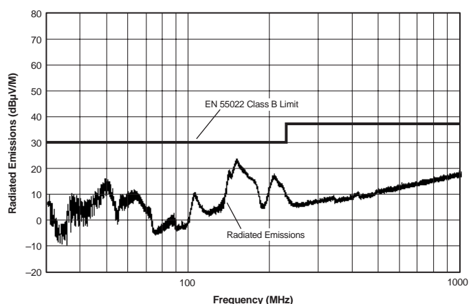
BWR-15/165-D48 Radiated Emissions EN 55022 Class B, 10 Meters Converter Output = \pm 15\text{Vdc} @ \pm 132\text{mA}
