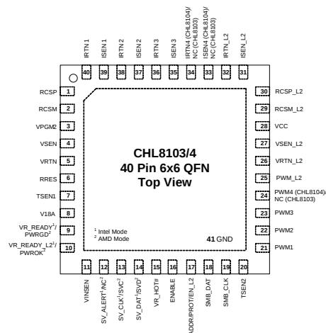
Figure 1: CHL8103/04 Package Top View
