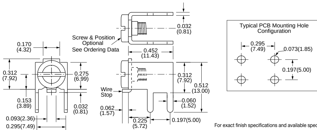
Typical PCB Mounting Configuration
