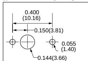
Typical PCB Mounting Configuration
