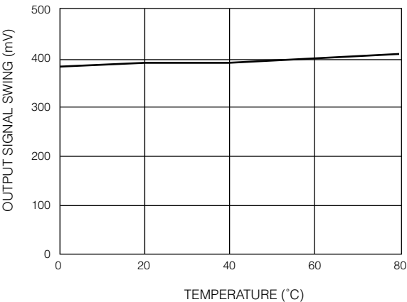
Fig. 18 Output Signal Swing, p-p, Differential
