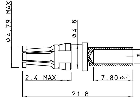
socket contact
