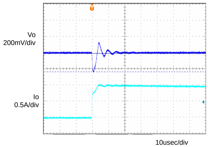
Fig.4 Transient Response (1.0→0A) Co=1\mu F , T_a=25^\circ C
