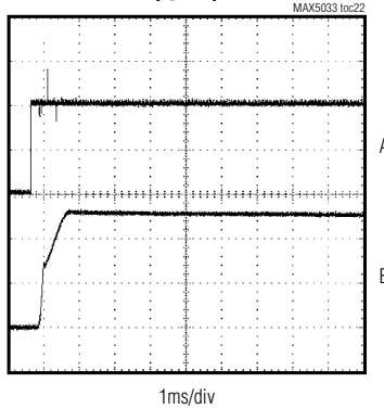
MAX5033BASA STARTUP WAVEFORM ( I_0 = 0 )
