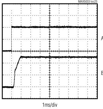
MAX5033BASA STARTUP WAVEFORM ( I_0 = 0.5A )
