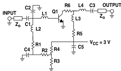
Figure 16. Schematic Diagram.
