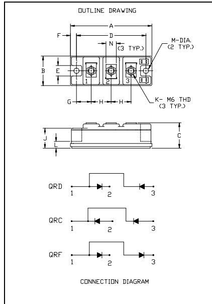
QR_1220T30 Fast Recovery Diode Module
