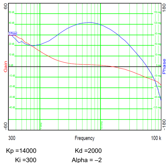
Figure 10-12. Bode Plot
