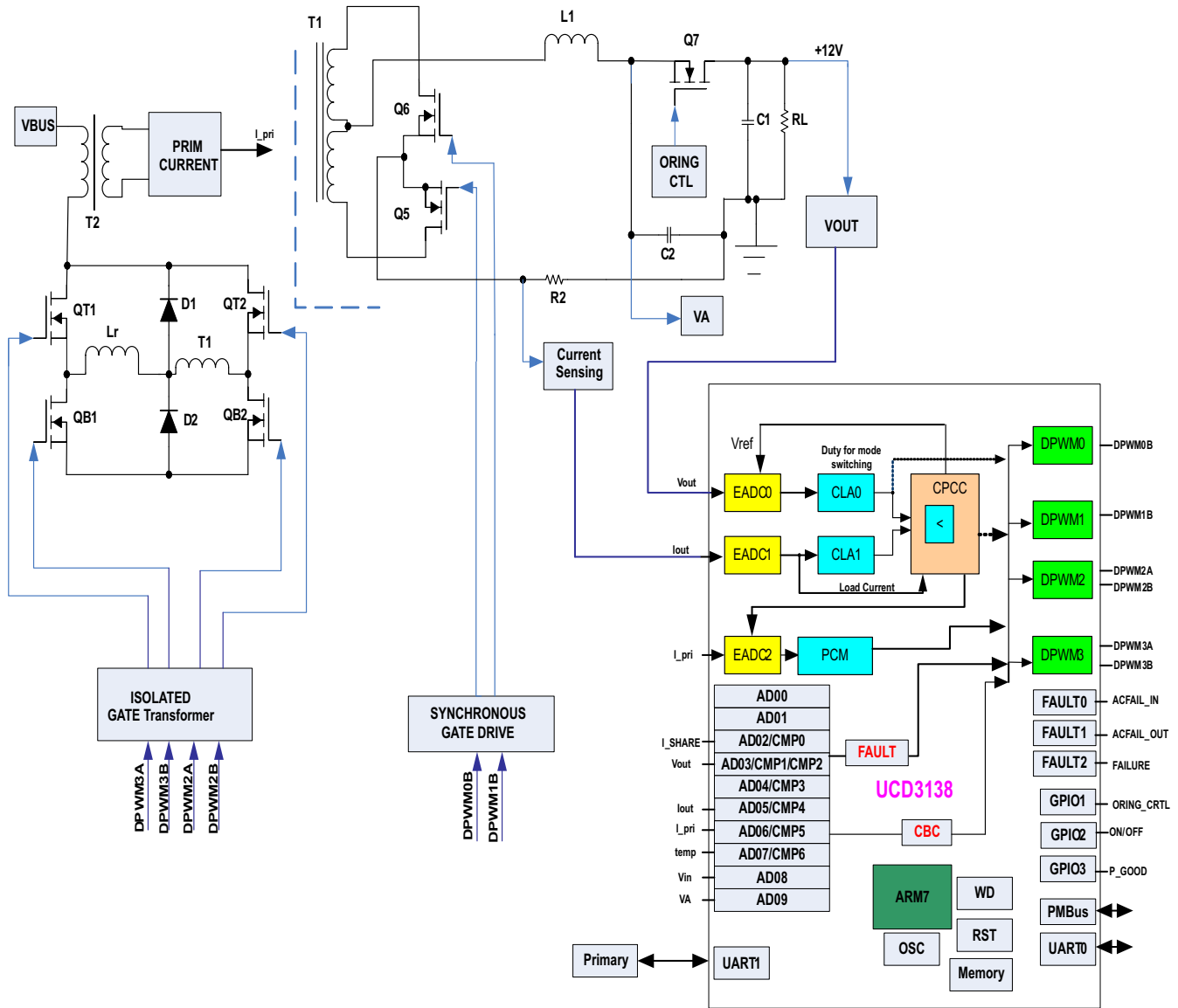
Figure 10-1. Phase-Shifted Full-Bridge
