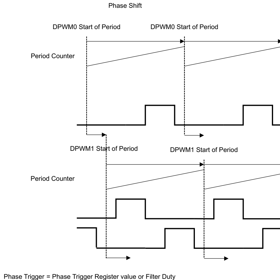
Figure 9-18. Phase Shift
