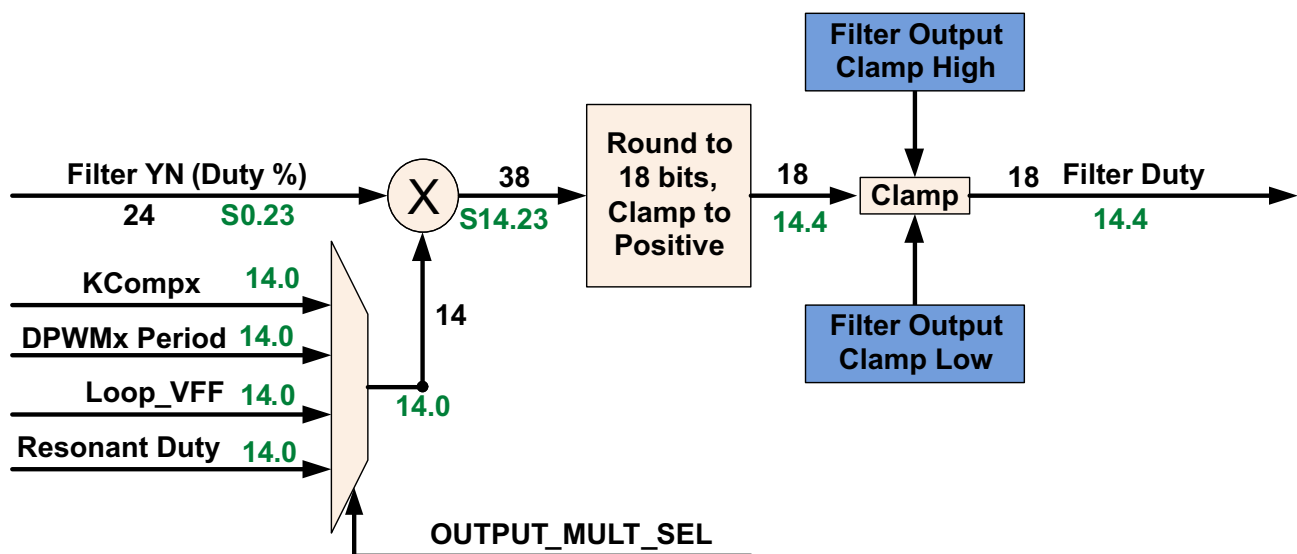
Figure 9-9. Resonant Mode
