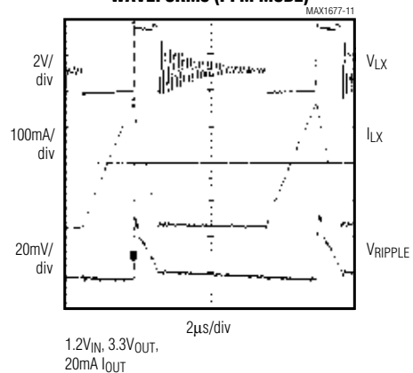
MAIN BOOST CONVERTER SWITCHING WAVEFORMS (PFM MODE)
