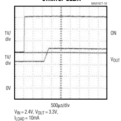
MAIN BOOST CONVERTER STARTUP DELAY
