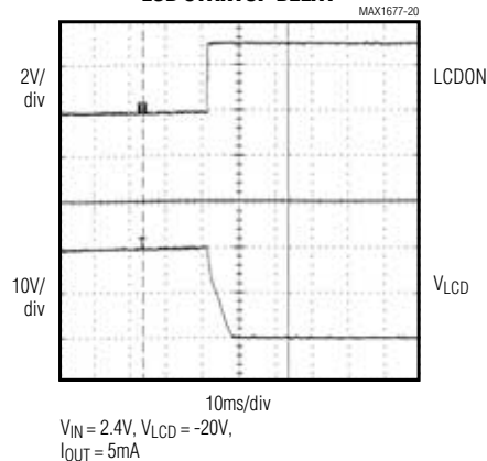
LCD STARTUP DELAY
