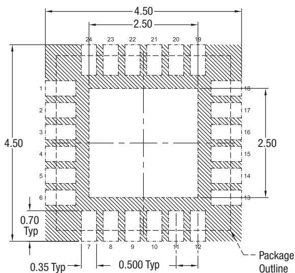
Solder Mask Pattern (Note 6)
