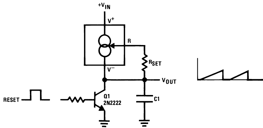
Ramp Generator
