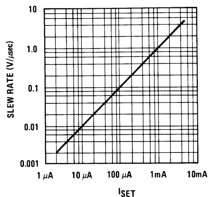
Maximum Slew Rate Linear Operation
