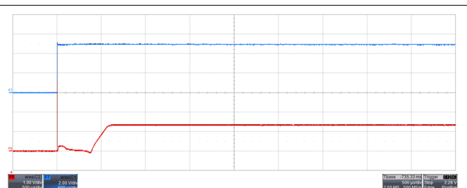
Figure 17. Output Turnon Response Time Without a Capacitive Load and V_{DD} = 5\text{ V}
