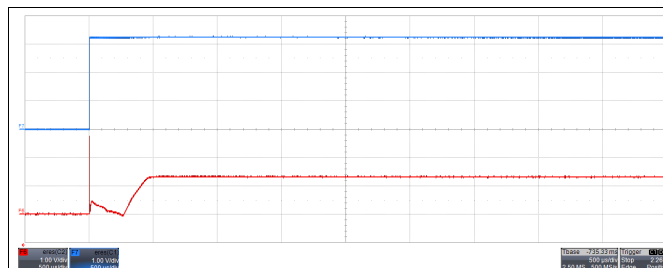
Figure 16. Output Turnon Response Time Without a Capacitive Load and V_{DD} = 3.3\text{ V}
