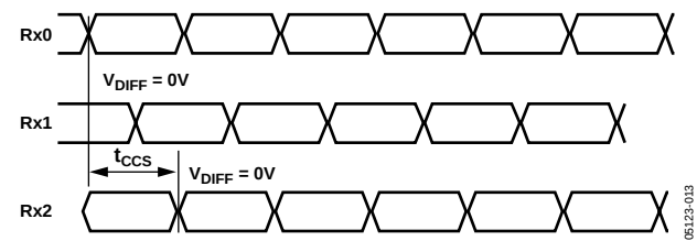
Figure 13. Digital Output Rise and Fall Times
