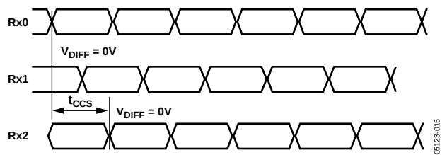
Figure 15. Channel-to-Channel Skew Timing
