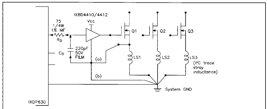
Fig. 11: Potential layout problems that create functional problems
