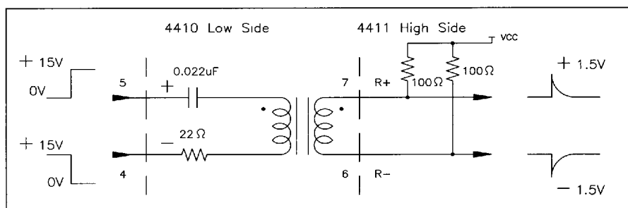
Fig. 13: Transmitter/Receiver Waveforms
