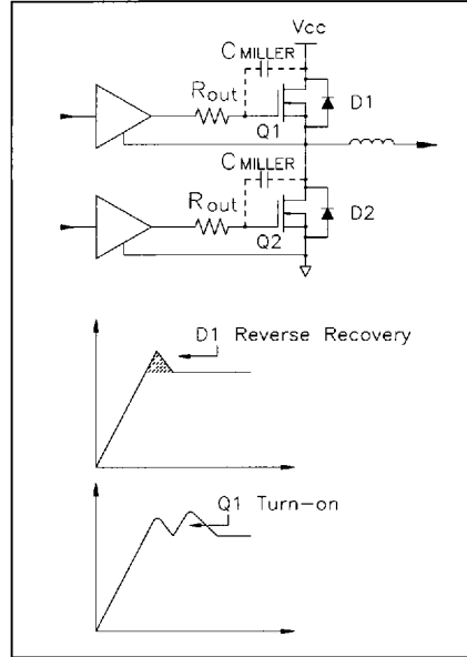
Fig. 5: Switching a clamped inductive load
