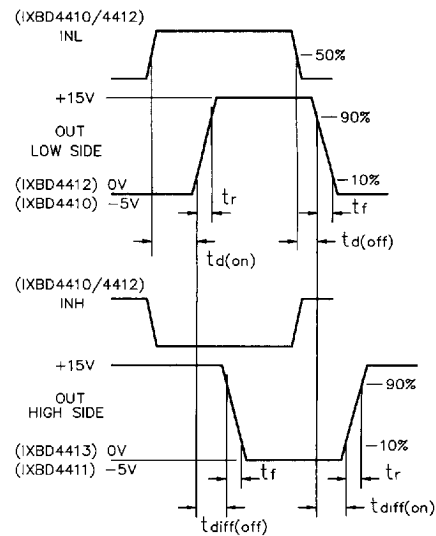
Fig. 1c: Output signal waveform
