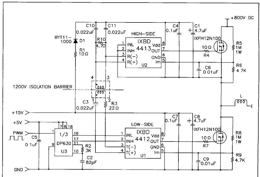
Fig. 9: Lower cost IXBD4412/4413 single phase circuit with deadtime generator IXDP630
