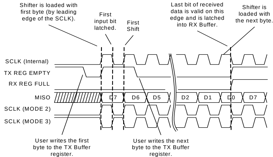
Figure 17-20. Typical SPI Timing in Modes 2 and 3
