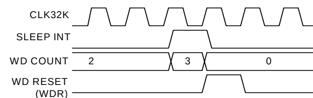
Figure 12-4. Watchdog Reset
