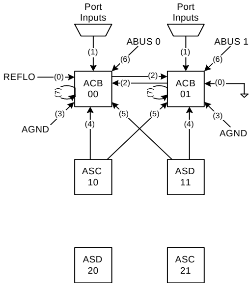
Figure 19-3. PMux Connections
