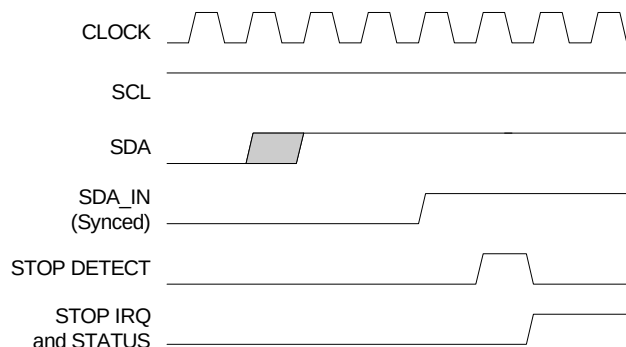
Figure 27-9. Stop Status and Interrupt Timing
