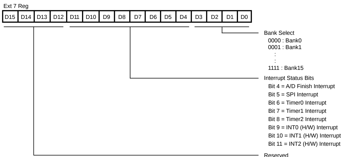
Figure 8. EXT7 Register Bit Assignment
