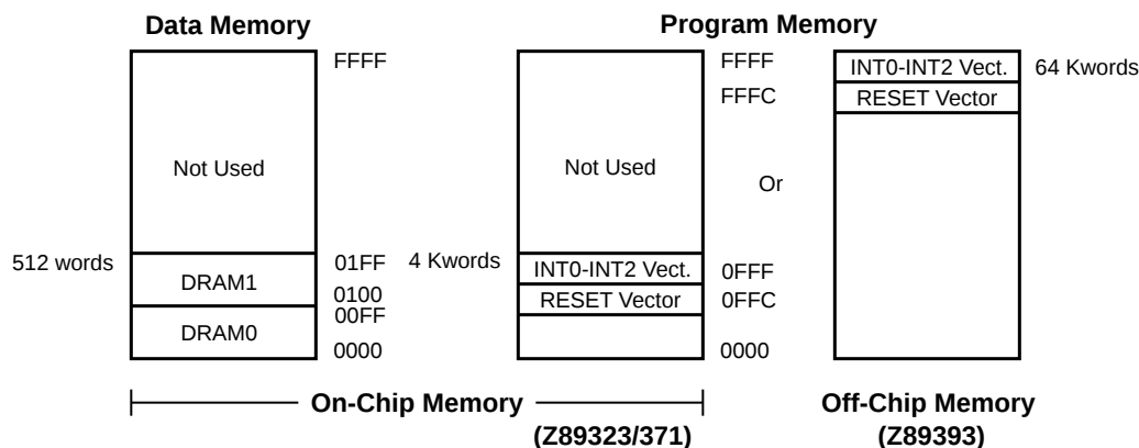
Figure 6. Memory Map
