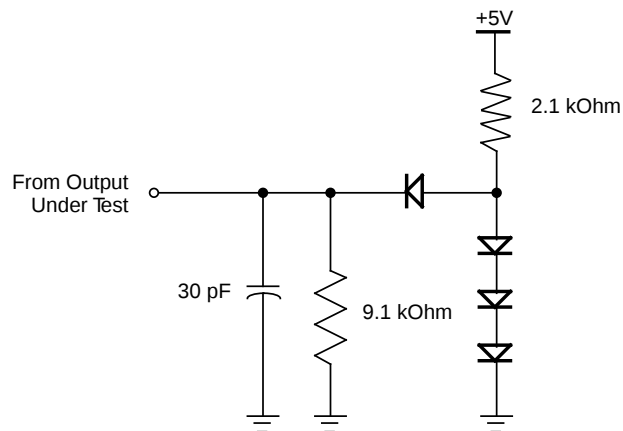
Figure 41. Test Load Diagram
