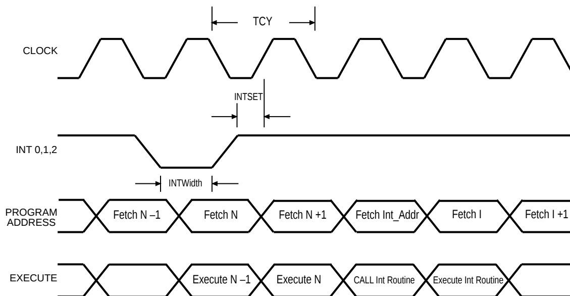
Figure 46. Interrupt Timing
