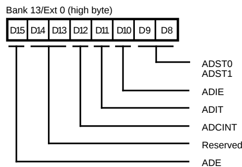
Figure 11. ADCTL Register (High Byte)
