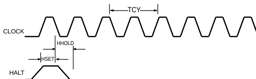
Figure 47. HALT Timing
