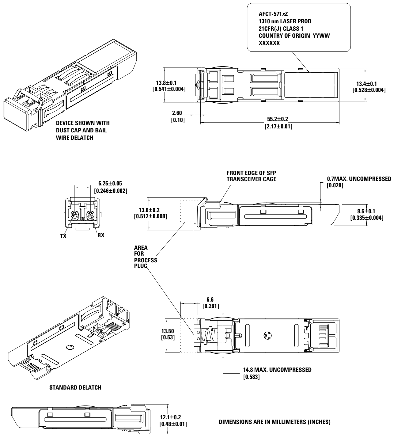
Figure 6. Drawing of SFP Transceiver
