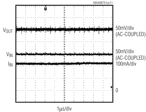
OPERATING WAVEFORMS 2X MODE
