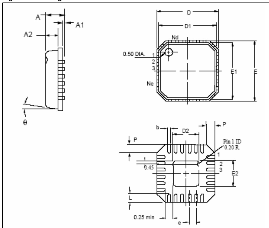
Figure 4. Package dimensions
