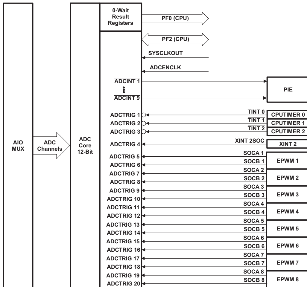
Figure 5-15. ADC Connections
