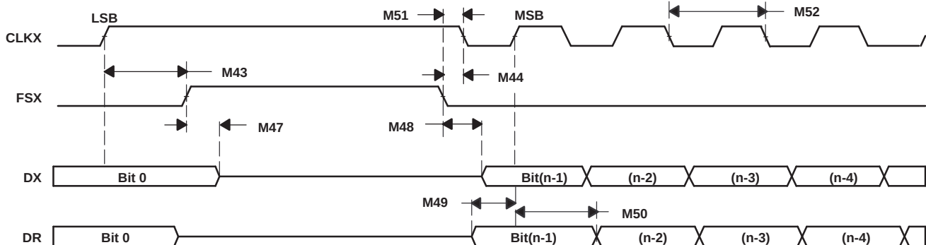
Figure 5-37. McBSP Timing as SPI Master or Slave: CLKSTP = 10b, CLKXP = 1
