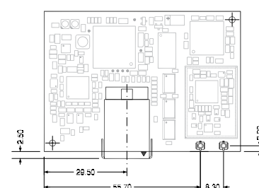
ConnectCore Wi-9P 9215 Top View
