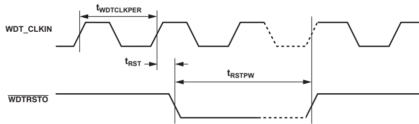
Figure 13. Watchdog Timer Timing
