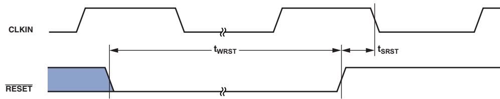
Figure 7. Reset
