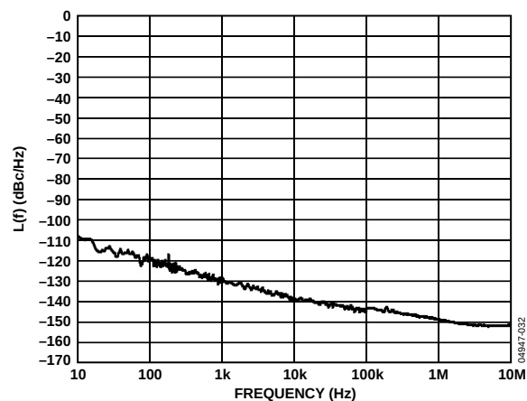
Figure 25. RF Divider and CML Driver Residual Phase Noise (1240 MHz In, 155 MHz Out)
