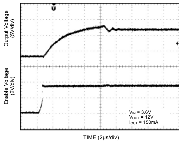
Enable Characteristics
