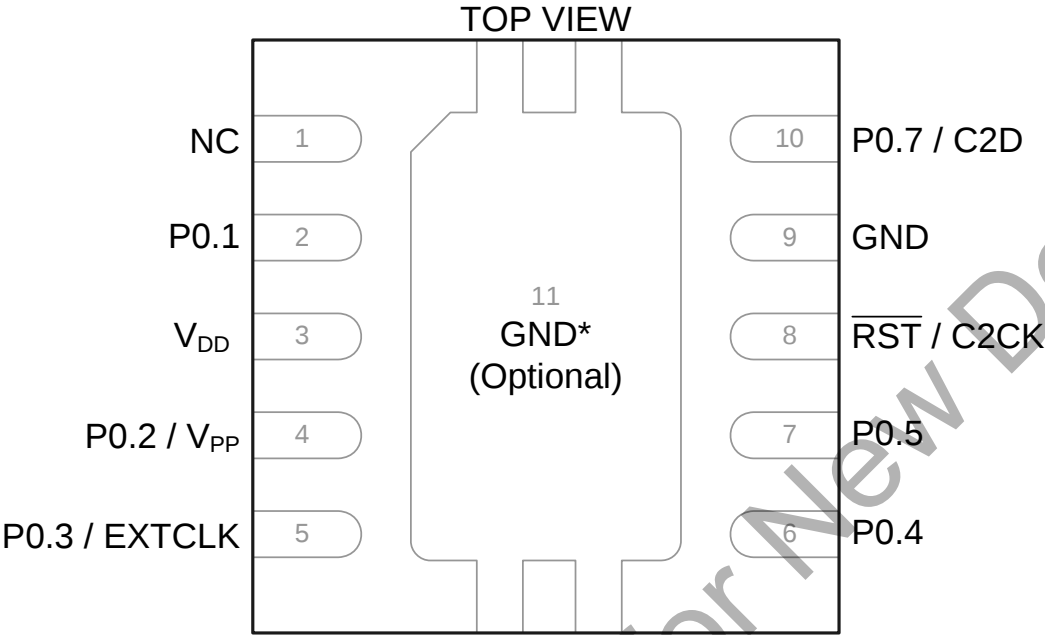
Figure 3.3. C8051T606-GM QFN11 Pinout Diagram (Top View)
