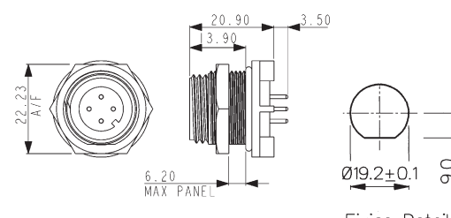
Fixing Details.
