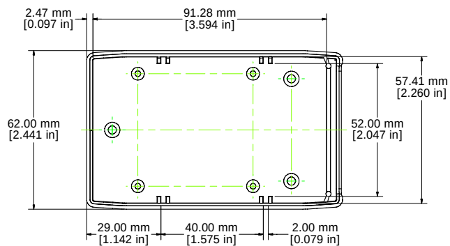
BOX - INSIDE
