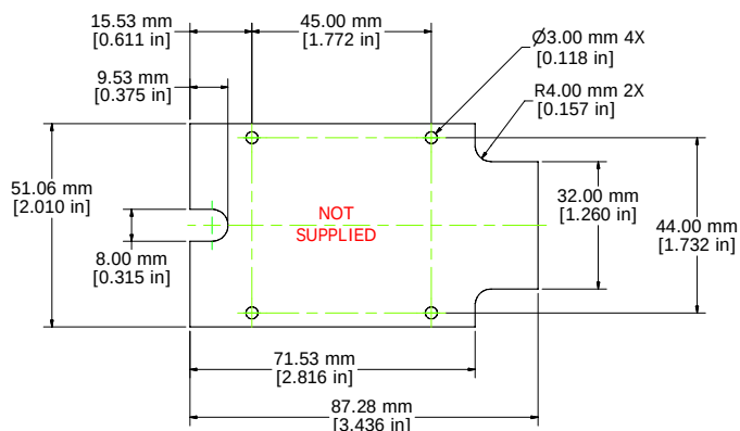
INNER PANEL
