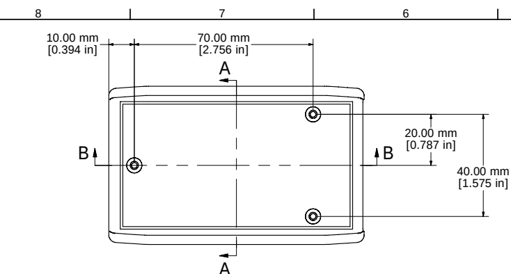
ASSEMBLY - TOP
