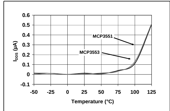
FIGURE 2-24: I_{DDS} vs. Temperature.
