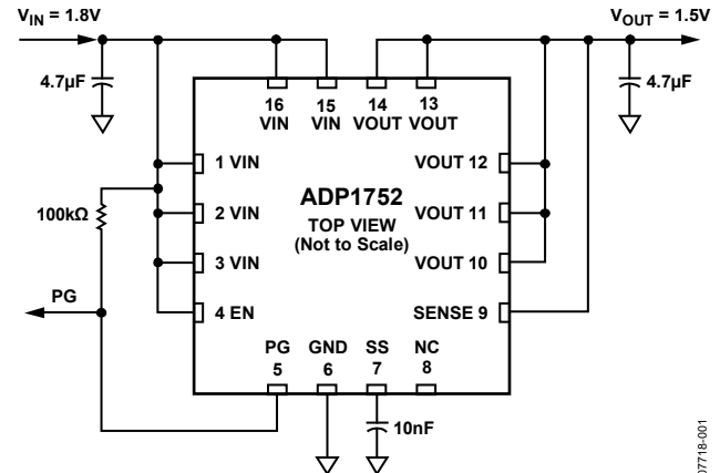
Figure 1. ADP1752 with Fixed Output Voltage, 1.5 V
