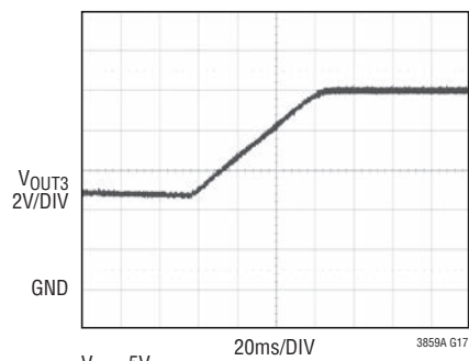
Soft Start-Up (Boost)
