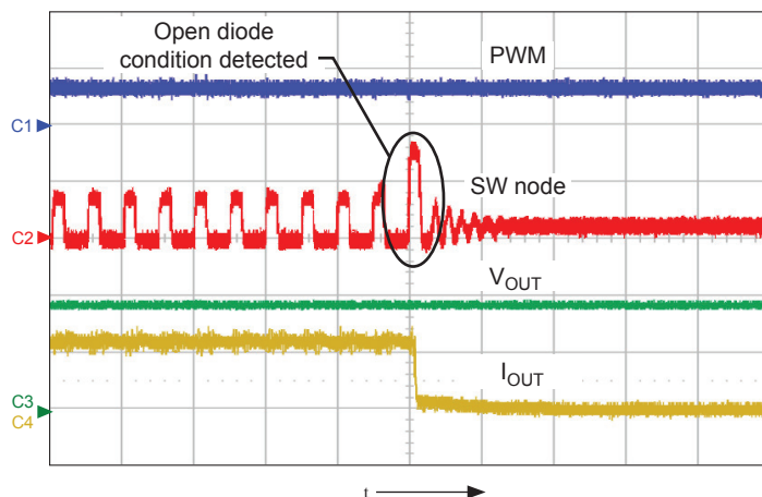
Figure 24. OVP protection in an open Schottky diode event, while the IC is in normal operation; shows PWM (ch1, 5 V/div.), SW node (ch2, 50 V/div.), V_{OUT} (ch3, 20 V/div.), and I_{OUT} (ch4, 200 mA/div.), time = 1 \mu s/div.
