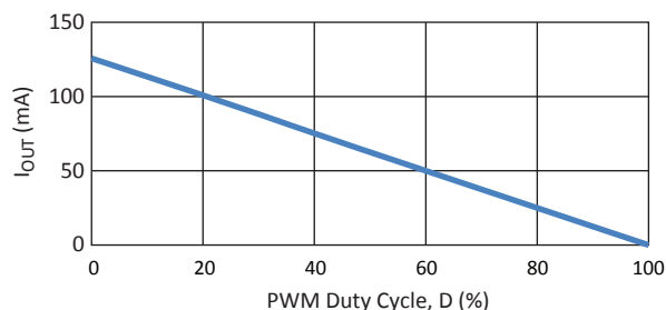
Figure 15. Output current versus duty cycle; 200 kHz APWM signal.
