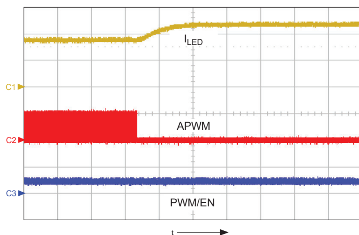
Figure 18. Diagram showing the transition of LED current from 90 mA to 120 mA, when a 25% duty cycle signal is removed from the APWM pin. PWM = 1; shows I_{LED} (ch1, 50 mA/div.), APWM (ch2, 5 V/div.), and PWM/EN (ch3, 5 V/div.), time = 500 \mu s/div.
