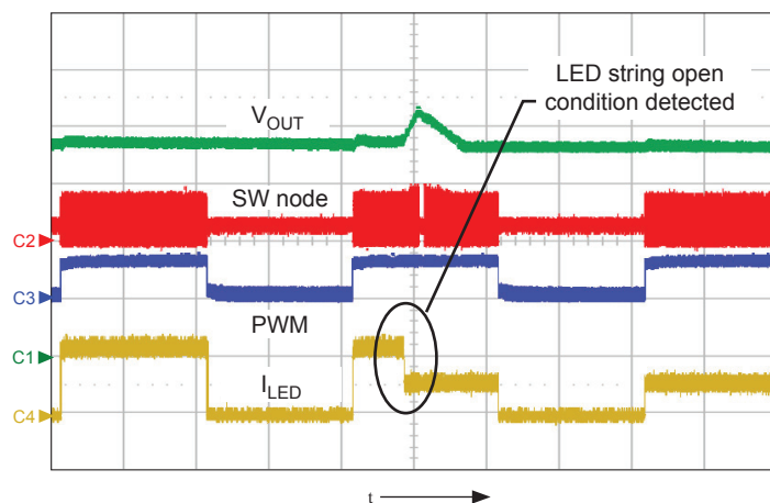
Figure 23. OVP protection in an open LED string event; shows V_{OUT} (ch1, 10 V/div.), SW node (ch2, 50 V/div.), PWM (ch3, 5 V/div.), and I_{LED} (ch4, 200 mA/div.), time = 500 \mu s /div.
