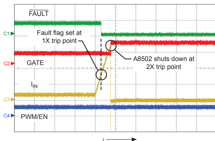
Figure 31. 2X mode, secondary overcurrent fault condition. I_{IN} is the input current through the switch. The Fault flag is set at the 1X current limit, and when the 2X current limit is reached the A8502 disables the gate of the disconnect switch (GATE); shows FAULT (ch1, 5 V/div.), GATE (ch2, 10 V/div.), I_{IN} (ch3, 2 A/div.), and PWM/EN (ch4, 5 V/div.), time = 5 \mu\text{s} /div.
