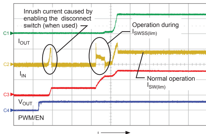
Figure 6. Startup diagram showing the input current, output current, and output voltage; shows I_{OUT} (ch1, 200 mA/div.), I_{IN} (ch2, 1 A/div.), V_{OUT} (ch3, 20 V/div.), and PWM/EN (ch4, 5 V/div.), time = 1 ms/div.
