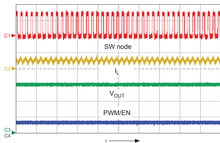
Figure 26. Normal operation of the switch node (SW); inductor current ( I_L ) and output voltage ( V_{OUT} ) for 9 series LEDs in each of 2 strings configuration; shows SW node (ch1, 20 V/div.), inductor current, I_L (ch2, 1 A/div.), V_{OUT} (ch3, 10 V/div.), and PWM/EN (ch4, 5 V/div.), time = 2 \mu s/div.
