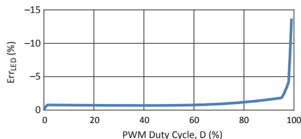
Figure 16. Percentage Error of the LED current versus PWM duty cycle; 200 kHz APWM signal.
