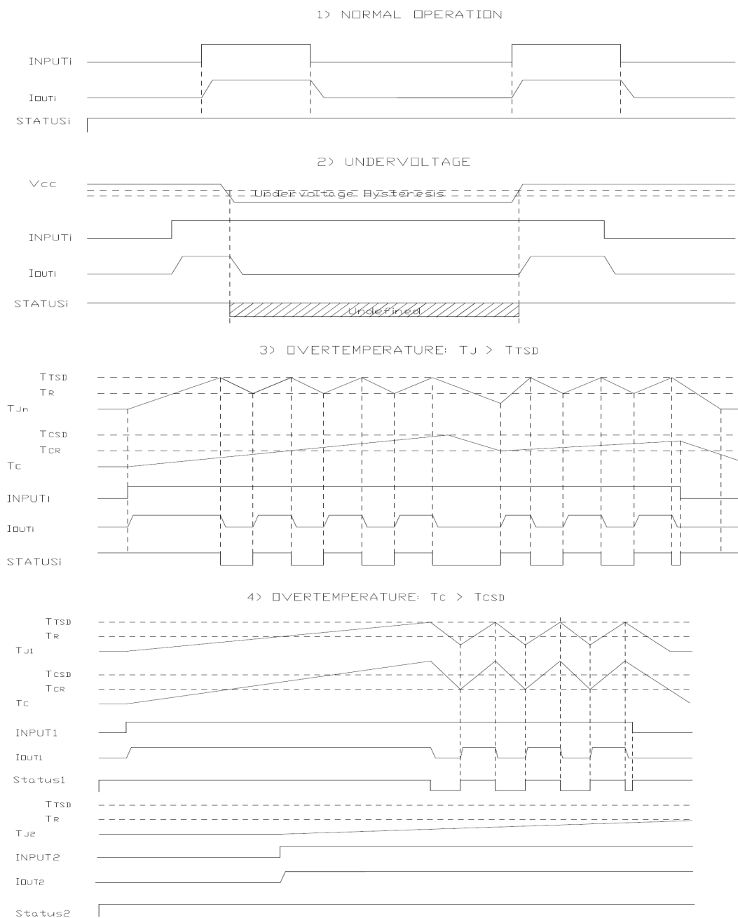
Figure 7. Switching waveforms
