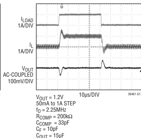
Load Step, Forced Continuous Operation
