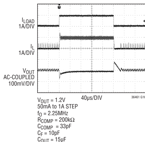
Load Step, Burst Mode Operation
