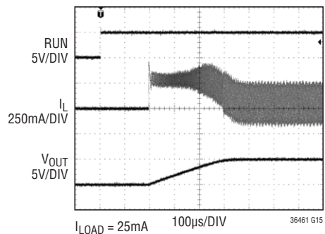
Start-Up from Shutdown, Forced Continuous Mode
