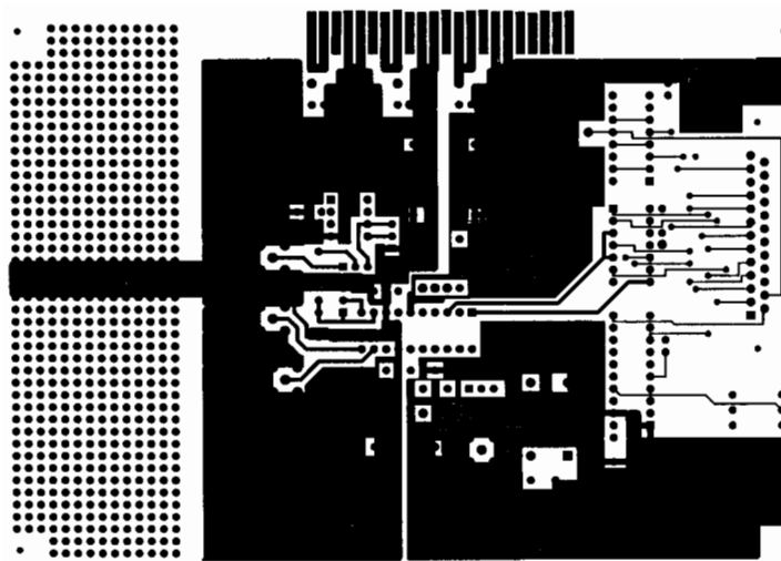
COMPONENT SIDE
