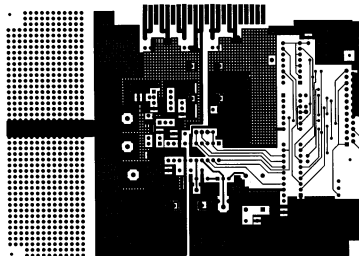
SOLDER SIDE
