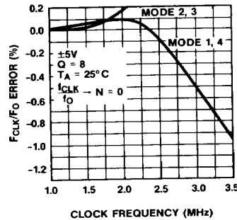
F_{CLK}/F_0 ERROR vs CLOCK FREQUENCY MAX261/2
