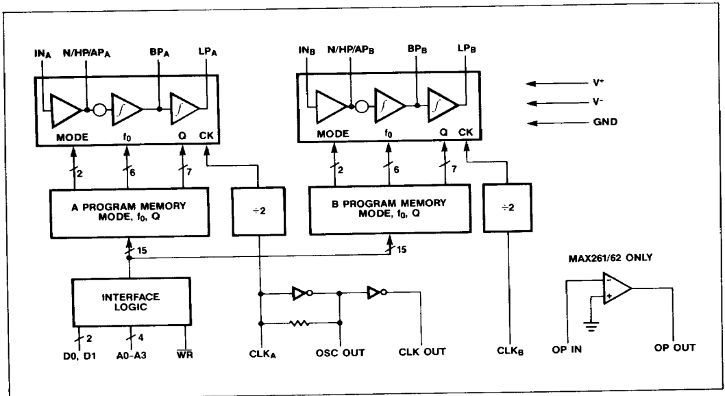
Figure 3. MAX260/61/62 Block Diagram
