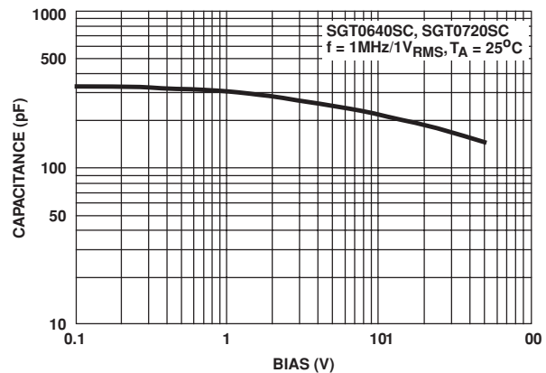
FIGURE 14. TYPICAL CAPACITANCE vs BIAS VOLTAGE
