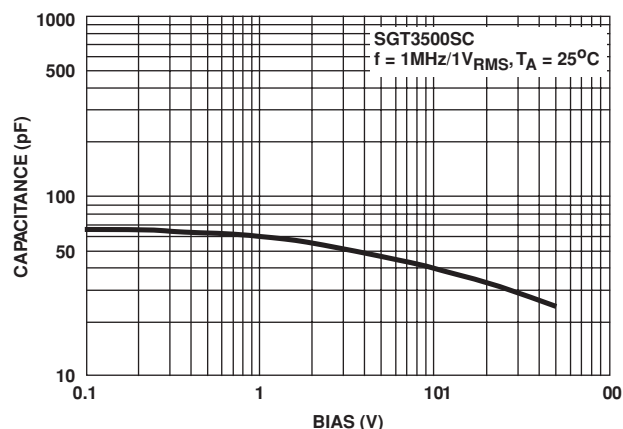
FIGURE 18. TYPICAL CAPACITANCE vs BIAS VOLTAGE
