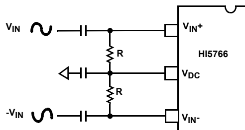
FIGURE 25. AC COUPLED DIFFERENTIAL INPUT
