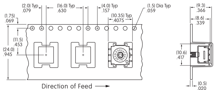
Tape Dimensions
