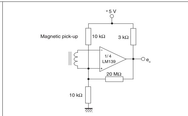
Figure 13. Transducer amplifier
