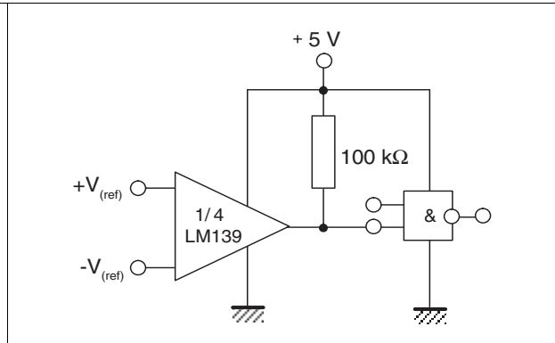
Figure 9. Driving CMOS
