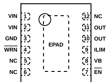
ISL9209B (12 LD 4x3 TDFN) TOP VIEW
