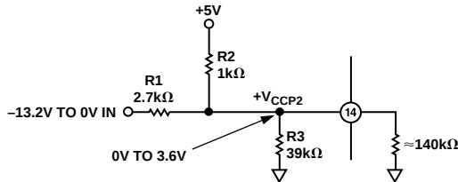
Figure 4. Scaling V_{CCP2} to -12\text{ V} ( \pm 10\% )
