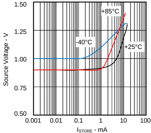
Minimum Start-Up Voltage vs STORE Output Current Circuit A with 10 \Omega Source Resistance (STORE=1.8V)
