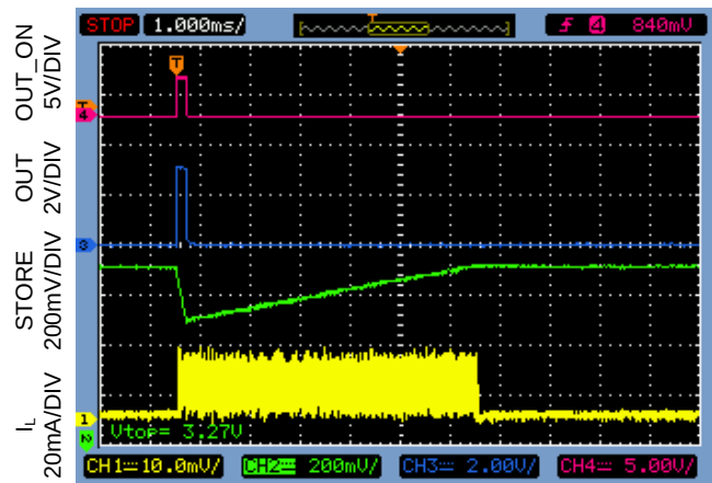
Figure 7. 220µF C_{STORE} Recovery Scope Capture
