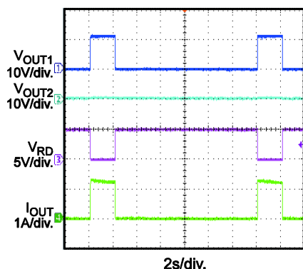
Locked-rotor Protection
