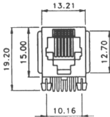
6P2C 6P4C 6P6C
