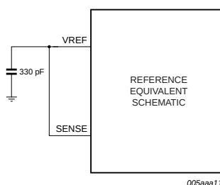
Fig 14. Internal reference via SPI, 1 V (p-p) to 2 V (p-p) full-scale
