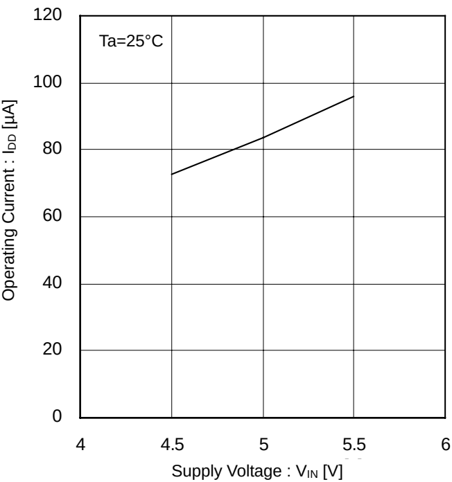
Figure 6. Operating Current vs Supply Voltage EN Enable
