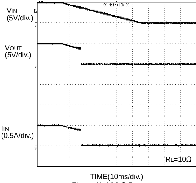
Figure 41. UVLO Response Decreasing V<sub>IN</sub>
