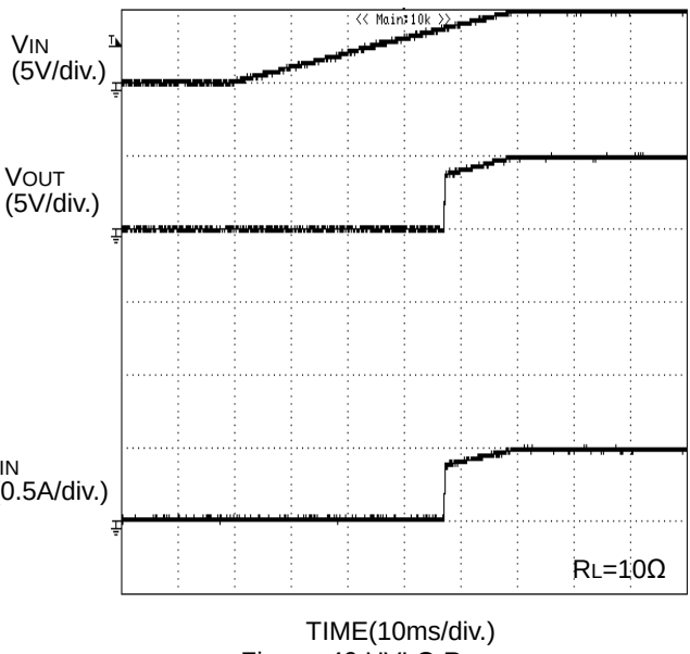
Figure 40. UVLO Response Increasing V<sub>IN</sub>
